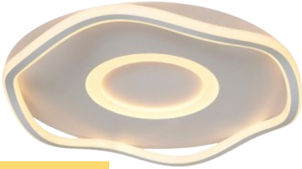
1435-03 KUMANDALI 28W LED Ø:40 H:10 3000-6500 Kelvin 2800 Lumen Metal, Acrylic
